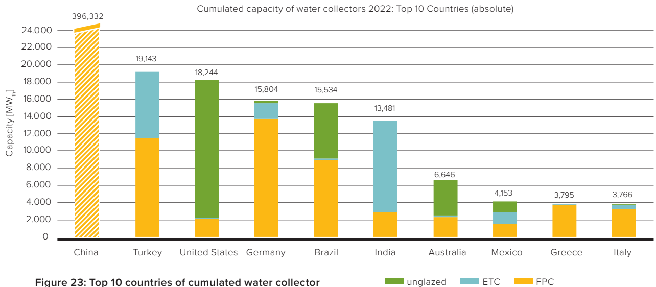
Figure 23: Top 10 countries of cumulated water collector installations in 2022 (absolute figures in MW th )
